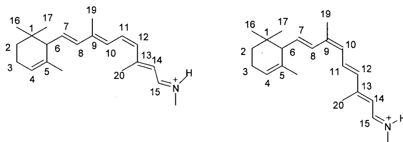
Figure 1. Structures and numbering of the chromophore in \alpha -rhodopsin and \alpha -isorhodopsin
