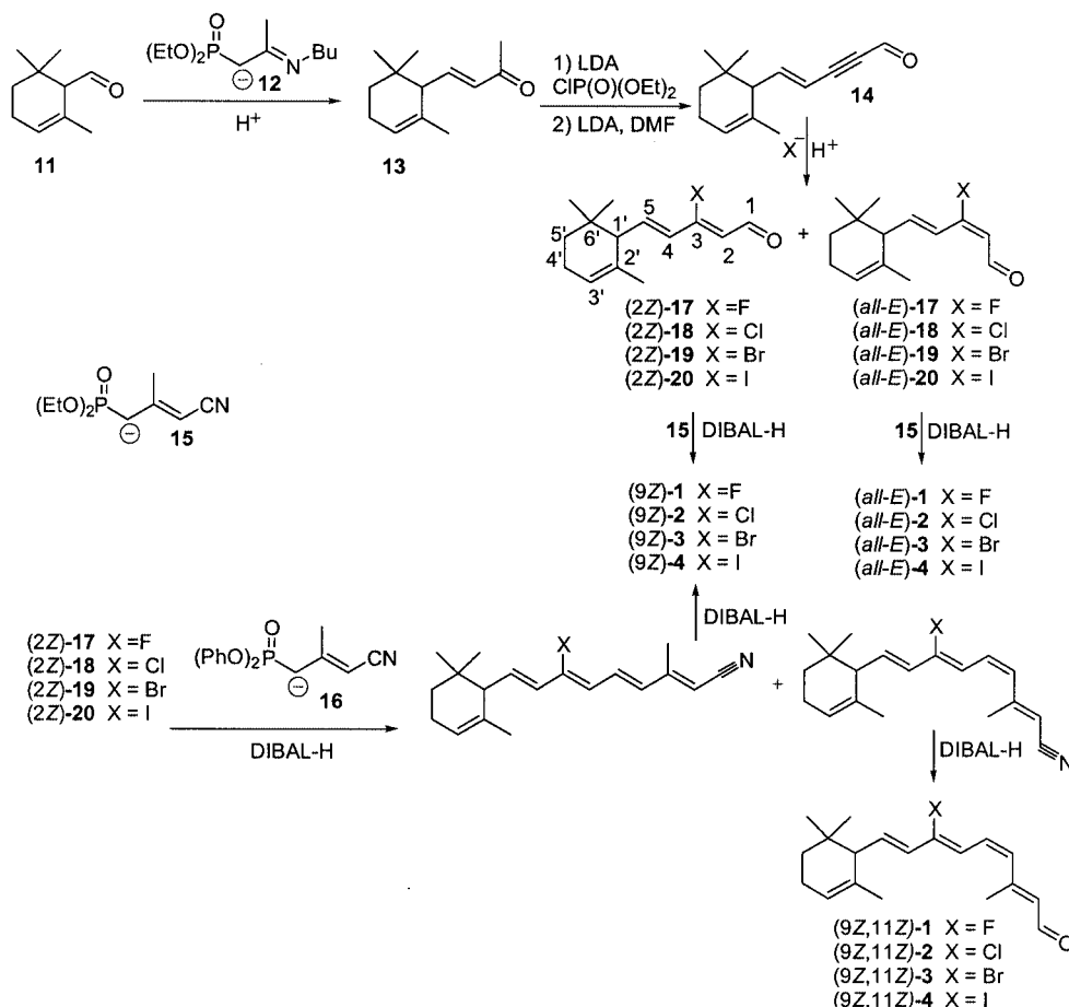
Scheme 1. Preparation of 9-demethyl-9-halo- \alpha -retinals in the pure ( all-E ), ( 9Z ), and ( 9Z,11Z ) isomeric forms
