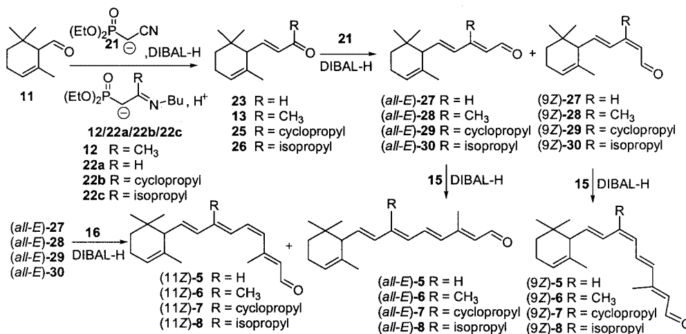
Scheme 2. Preparation of 4,5-didehydro-9-demethyl-5,6-dihydroretinal ( 5 ), 4,5-didehydro-5,6-dihydro-9-methylretinal ( 6 ), 4,5-didehydro-19,19-ethano-5,6-dihydroretinal ( 7 ) and 4,5-didehydro-5,6-dihydro-19,19-dimethylretinal ( 8 ) in (all-E), (9Z), and (11Z) isomeric forms; for the preparation of 9 and 10 in the (all-E), (9Z), and (11Z) isomeric forms the corresponding \beta -derivatives are used
